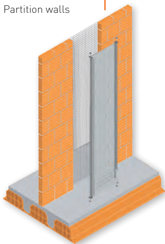
Partition walls
