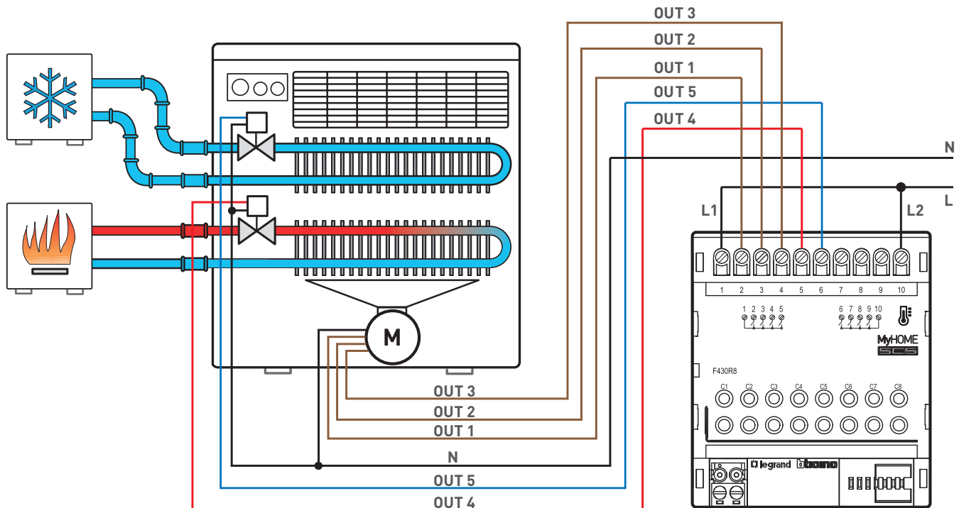
Use of the F430/8 actuator, for the control of a 4-tube and 3-speed fan-coil.
