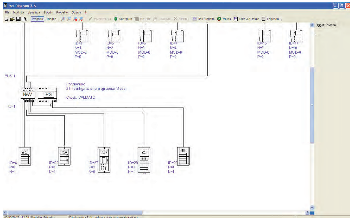
Example of a video door entry system design
