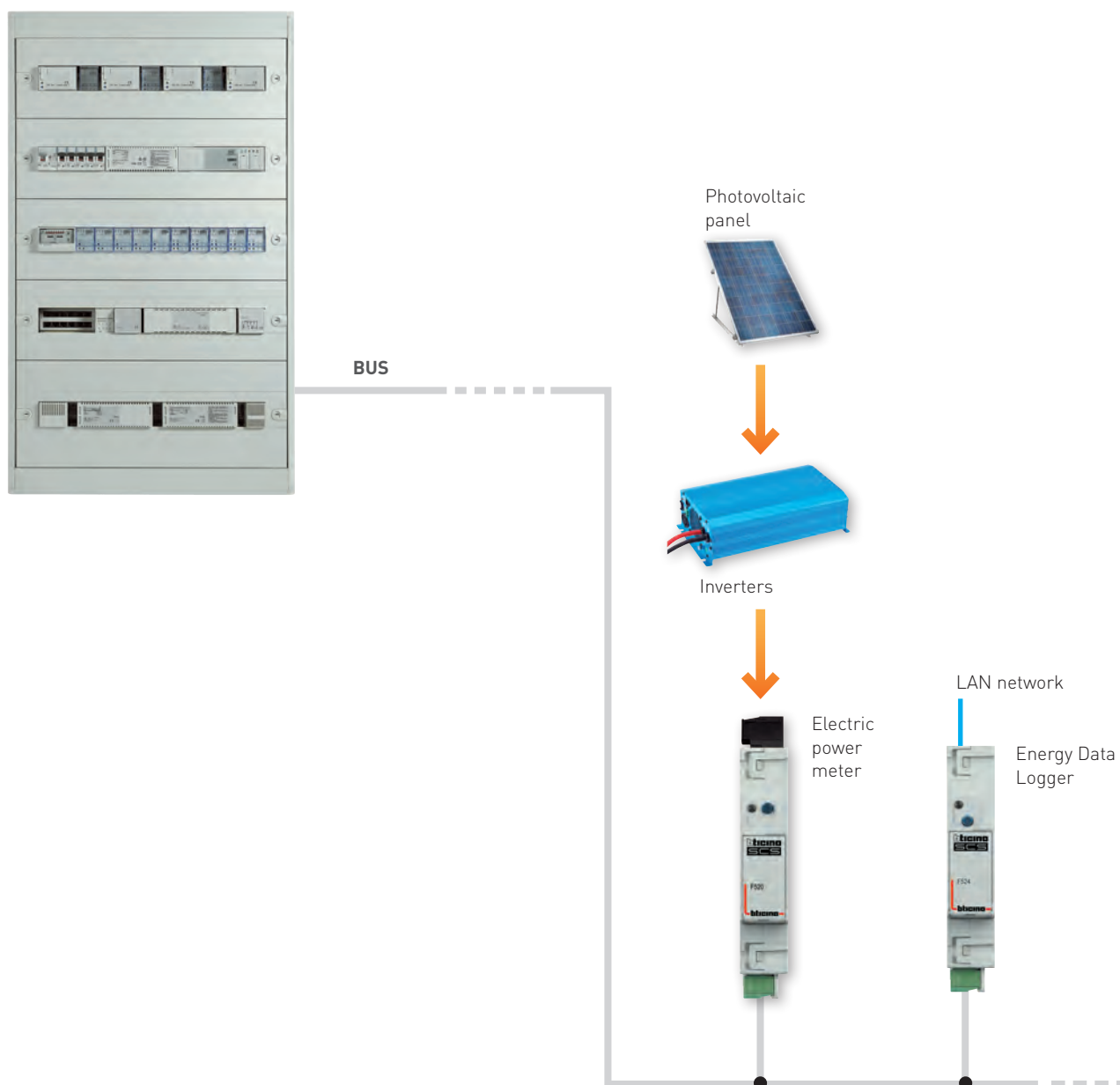
Switchboard
