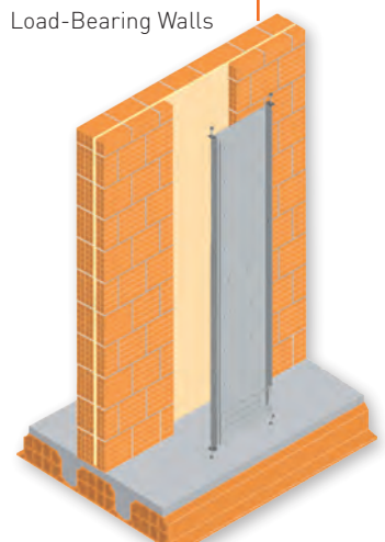
Load-Bearing Walls
