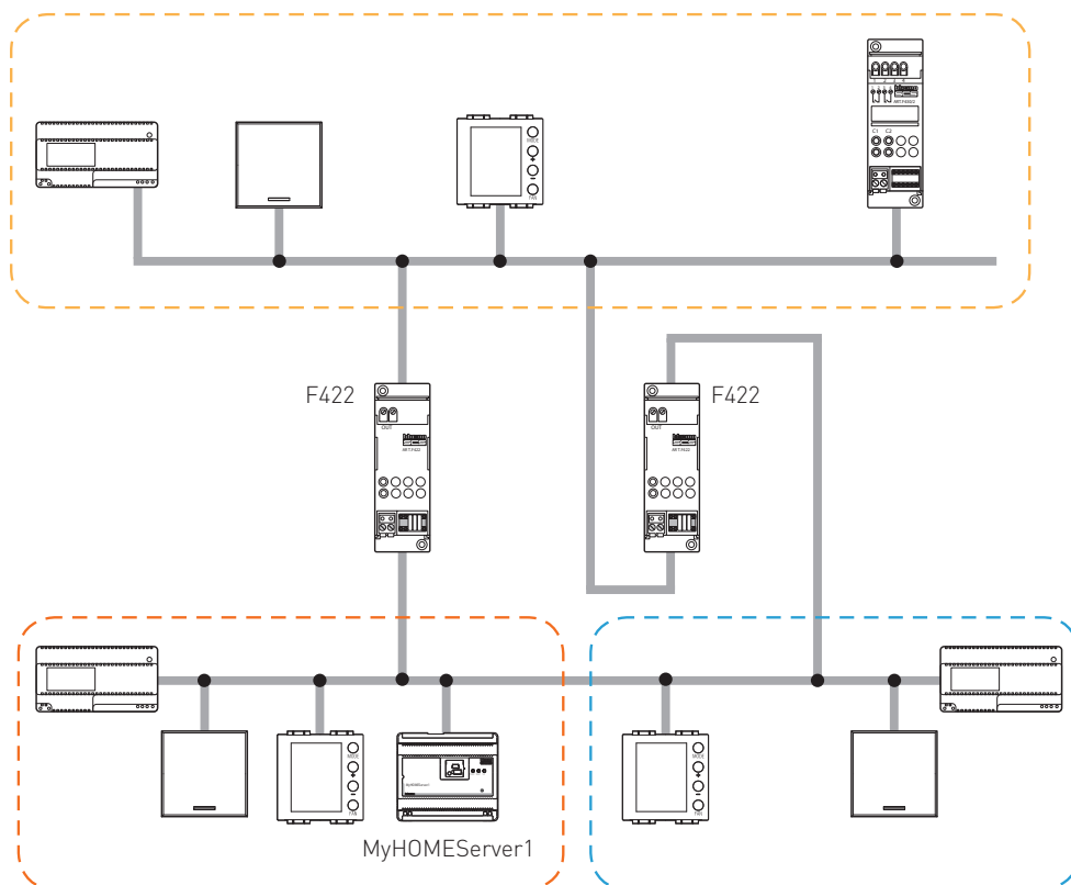
Example of temperature control system integrated with the light and shutter automation system.
