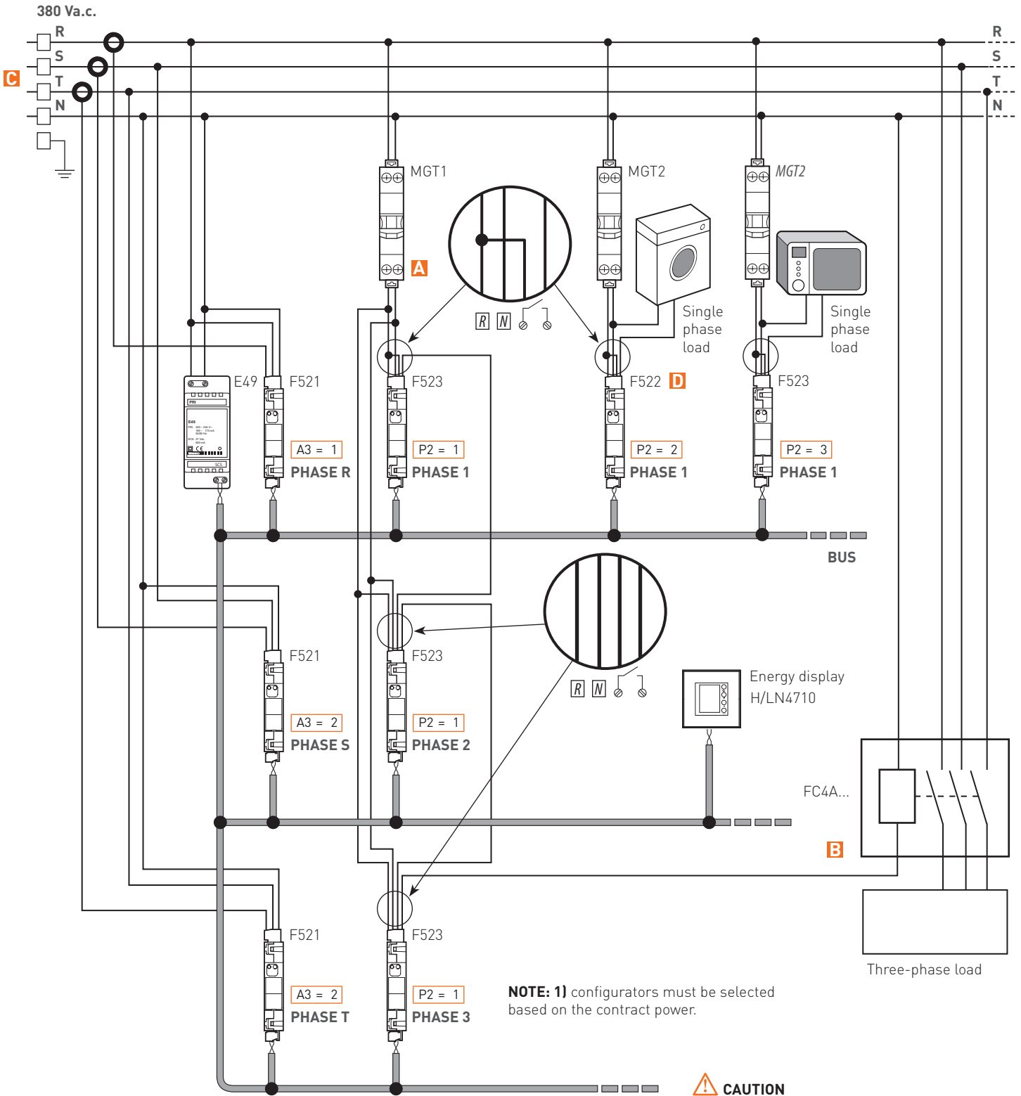
DIAGRAM 2 - THREE-PHASE LOAD CONTROL MANAGEMENT AND SINGLE PHASE LOAD WITH BUS SCS IN COMMON
