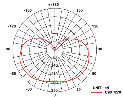
AVERAGE BEAM ANGLE (50%) : 262.1 DEG LUMINOUS INTENSITY DISTRIBUTION DIAGRAM
