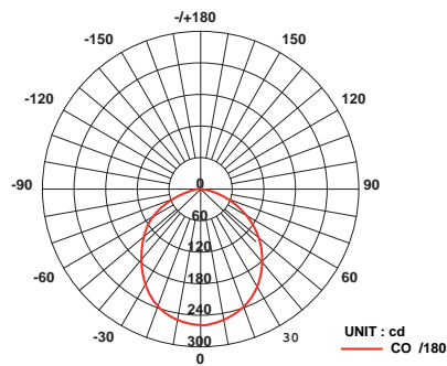
AVERAGE BEAM ANGLE (50%) : 107.6 DEG LUMINOUS INTENSITY DISTRIBUTION DIAGRAM
