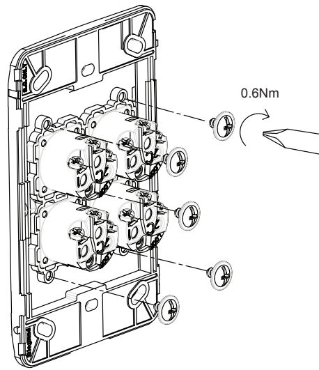
4 Gang switch grid
