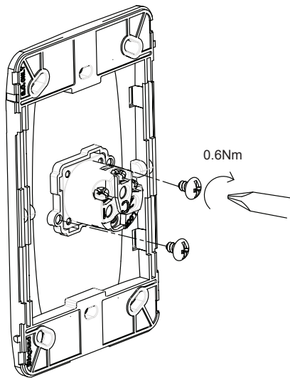
1-3 Gang switch grid
